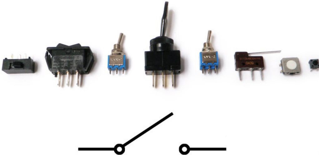
Figure 1.2.1 (L) Switches
