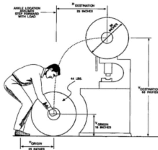
Figure. 2.4.3. NIOSH Lifting Equation applied to loading punch press stock task
